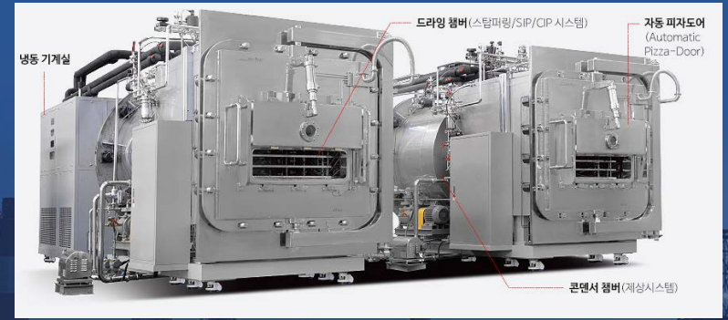
Freeze dryer
